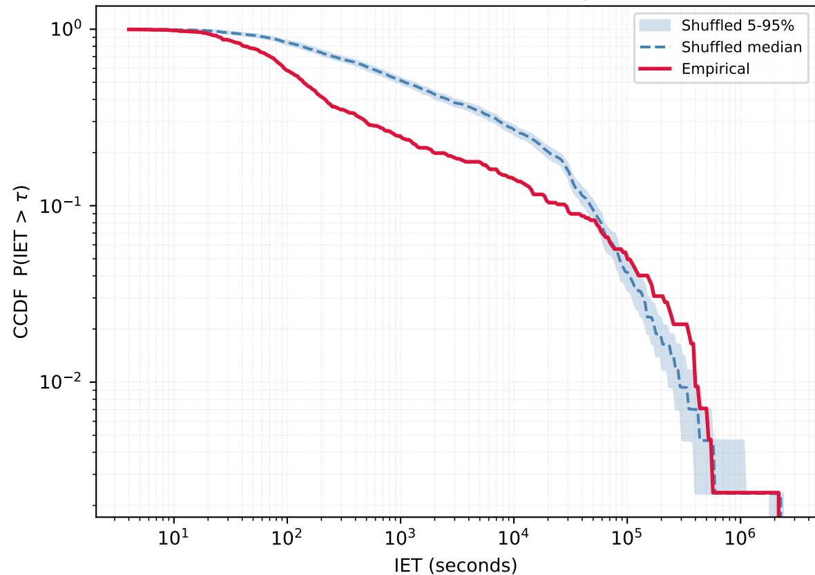
User 7094531229 - Empirical vs Reshuffled | KS=0.341 p=0.000
